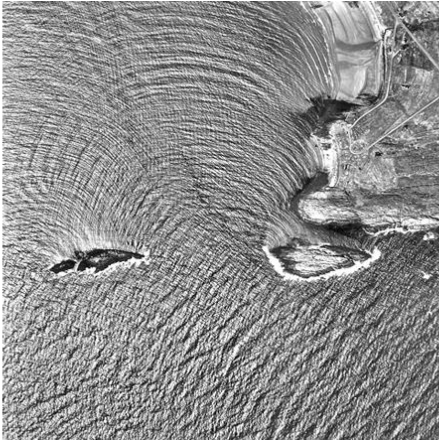
Diffraction and interference in water waves
