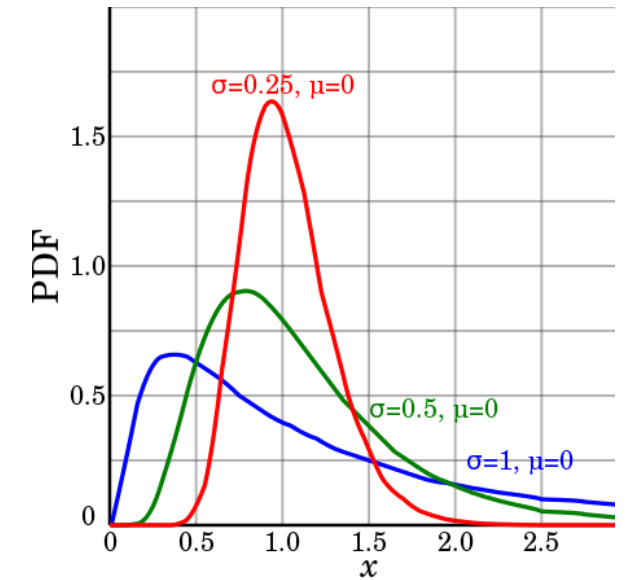
Log-normal distribution
