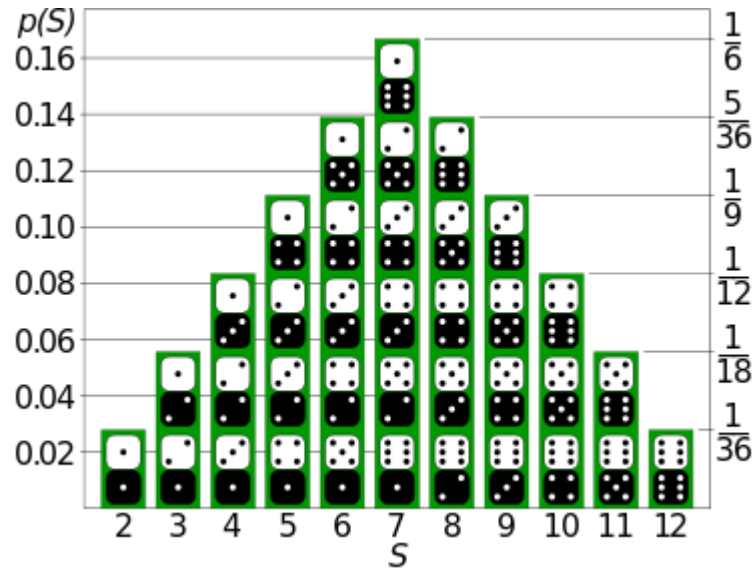
Discrete – sum of two dice
