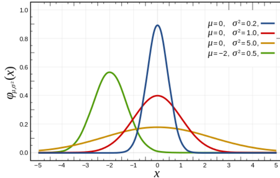
Normal (Gaussian) distribution
